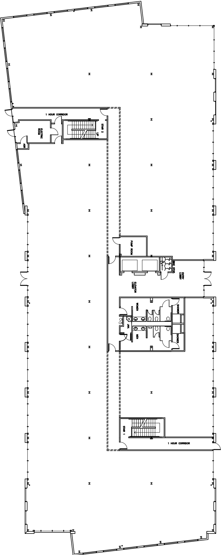
FIRST FLOOR PLAN REDWOOD BUSINESS CENTER
